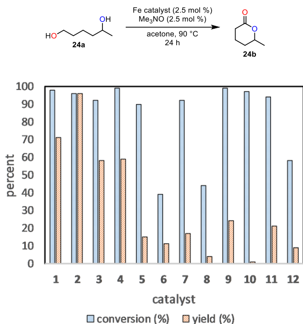
Figure 4. Lactonization of 1,5-hexanediol with (cyclopentadienone)iron tricarbonyl catalysts. Reaction conditions: 1,5-hexanediol (1 equiv, 0.5 M in acetone), Fe catalyst (0.025 equiv), anhydrous trimethylamine N -oxide (0.025 equiv), biphenyl (0.25 equiv), and acetone at 90 °C for 24 h in a sealed, thick-walled test tube. Diol conversion and lactone yield determined by gas chromatography relative to biphenyl.
