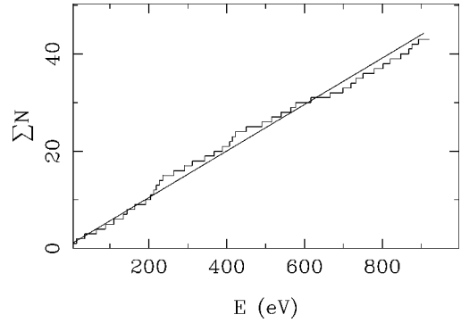
FIG. 3. Cumulative number of levels for 133 Cs s -wave resonances. A linear fit was used to extract the s -wave level spacing.
