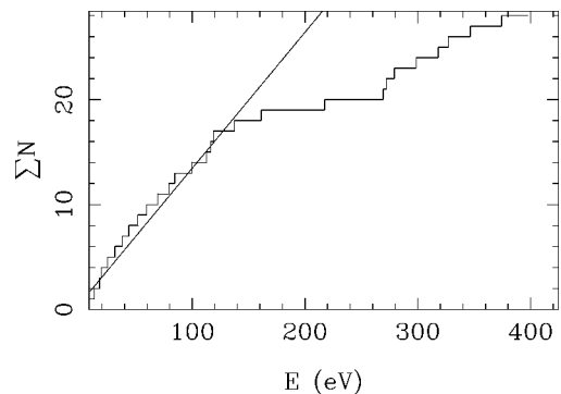
FIG. 4. Cumulative number of levels for 133 Cs p -wave resonances. The linear fit indicates that some levels are missed above 120 eV.
