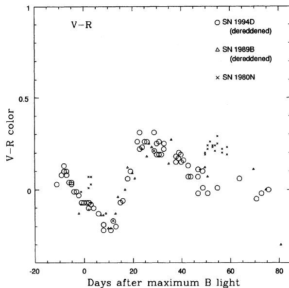
FIG. 13. (V-R) color curves of SNe 1994D, 1980N, and 1989B. The data for SN 1994D have been dereddened by -0.03 mag. The data for SN 1989B have been dereddened by -0.30 mag (W94).
