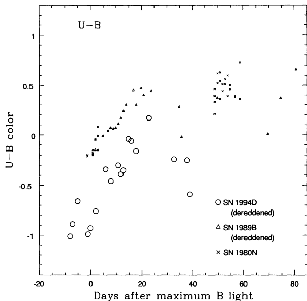
FIG. 11. (U-B) color curves of SNe 1994D, 1980N, and 1989B. The data for SN 1994D have been dereddened by -0.04 mag. The data for SN 1989B have been dereddened by -0.29 mag (W94). The U -band measurements for SN 1994D may be systematically too bright by up to 0.5 mag.
