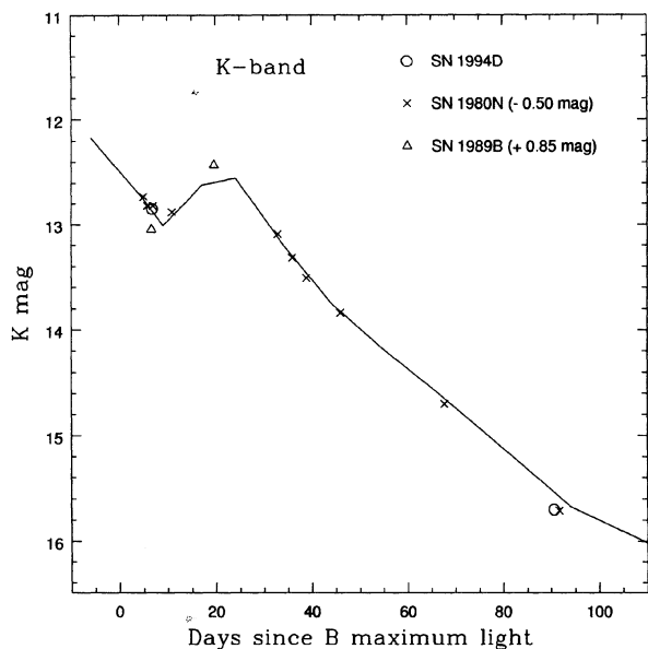
FIG. 17. K -band light curves for SNe 1994D, 1980N, and 1989B. Note that the second datum for SN 1994D was taken at K'=2.1 μm. The line shows the template curve for type Ia SNe of Elias et al. (1985). The data for SN 1989B have been dereddened following W94.
