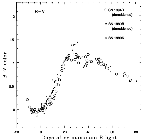
FIG. 12. (B-V) color curves of SNe 1994D, 1980N, and 1989B. The data for SN 1994D have been dereddened by -0.04 mag. The data for SN 1989B have been dereddened by -0.37 mag (W94).
